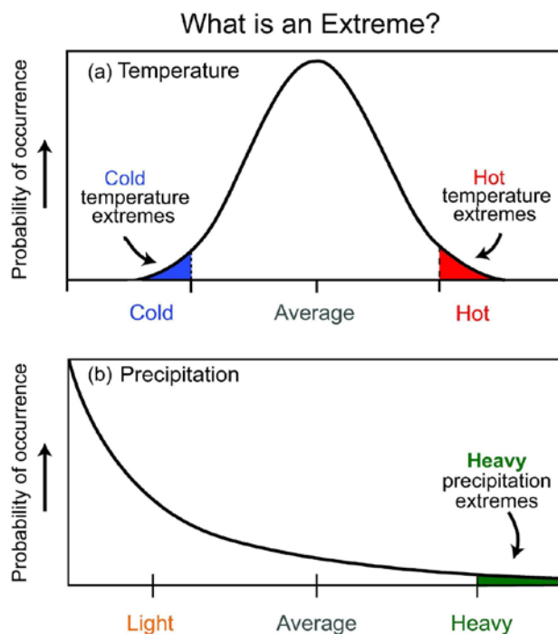
Figure 1: Schematic representations of the probability distributions of daily temperature, which tends to be approximately Gaussian (exceptions can be caused by soil freezing, feedbacks, or energy balance constraints, see text), and daily precipitation, which has a skewed distribution. Extremes are denoted by the shaded areas. In the case of temperature, changes in the frequencies of extremes are strongly affected by changes in the mean; a relatively small shift of the distribution to the right would substantially increase warm extremes and decrease cold extremes. In addition, the frequency of extremes can also be affected by changes in the shape of the tails of the temperature distribution, which could become wider or narrower, or could become somewhat skewed rather than being symmetric as depicted. In a skewed distribution such as that of precipitation, a change in the mean of the distribution generally affects its variability or spread, and thus an increase in mean precipitation would also likely imply an increase in heavy precipitation extremes, and vice-versa. In addition, the shape of the right hand tail could also change, affecting extremes. Furthermore, climate change may alter the frequency of precipitation and the duration of dry spells between precipitation events. From Folland et al (1995) and Peterson et al (2008).
