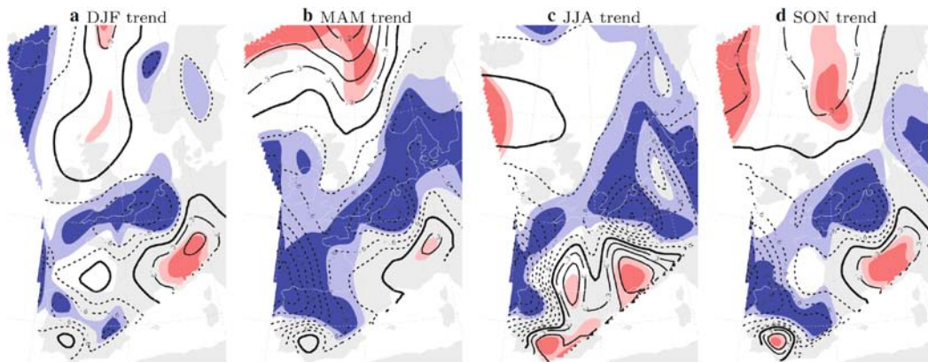
Figure 5: Example of an analysis of trends in seasonal storm indices derived from long surface pressure records. This figure shows contour maps of Theil-Sen (also sometimes know as Kendall's) linear trend estimates (in unit per century) in seasonal storm indices defined as the 99 th percentile of sub-daily geostrophic wind speed estimated from pressure triangles for the period 1902–2007 in a domain the covers western Europe and the eastern North Atlantic. The contour interval is 0.3. The zero contours are shown in bold. Positive trends are shown in thin solid contours, and reddish shadings indicate at least 20% significance; and negative trends in dashed contours and bluish shadings. The darker shadings indicate areas with trends that are significant at the 5% level or lower. Significance is determined using the Mann-Kendall trend test. From Wang et al (2011). The statistical methods are described in Wang and Swail (2001).
