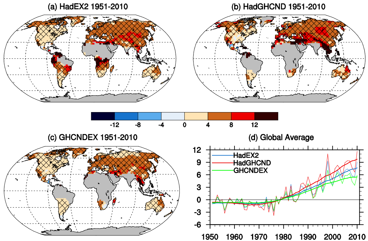
Figure 2: Annual trends in warm nights (TN90p) using different datasets for the period 1951 to 2010 where at least 40 years are available. The datasets are (a) HadEX2 (Alexander and Donat 2011), (b) HadGHCNDEX (ETCCDI indices calculated from an updated version of HadGHCND (Caesar et al. 2006)) and (c) GHCNDEX (Donat and Alexander, 2011). Panel (d) represents the global average time series plots for each of the three datasets presented as anomalies relative to the 1961-1990 with associated 21-year Gaussian filters.
